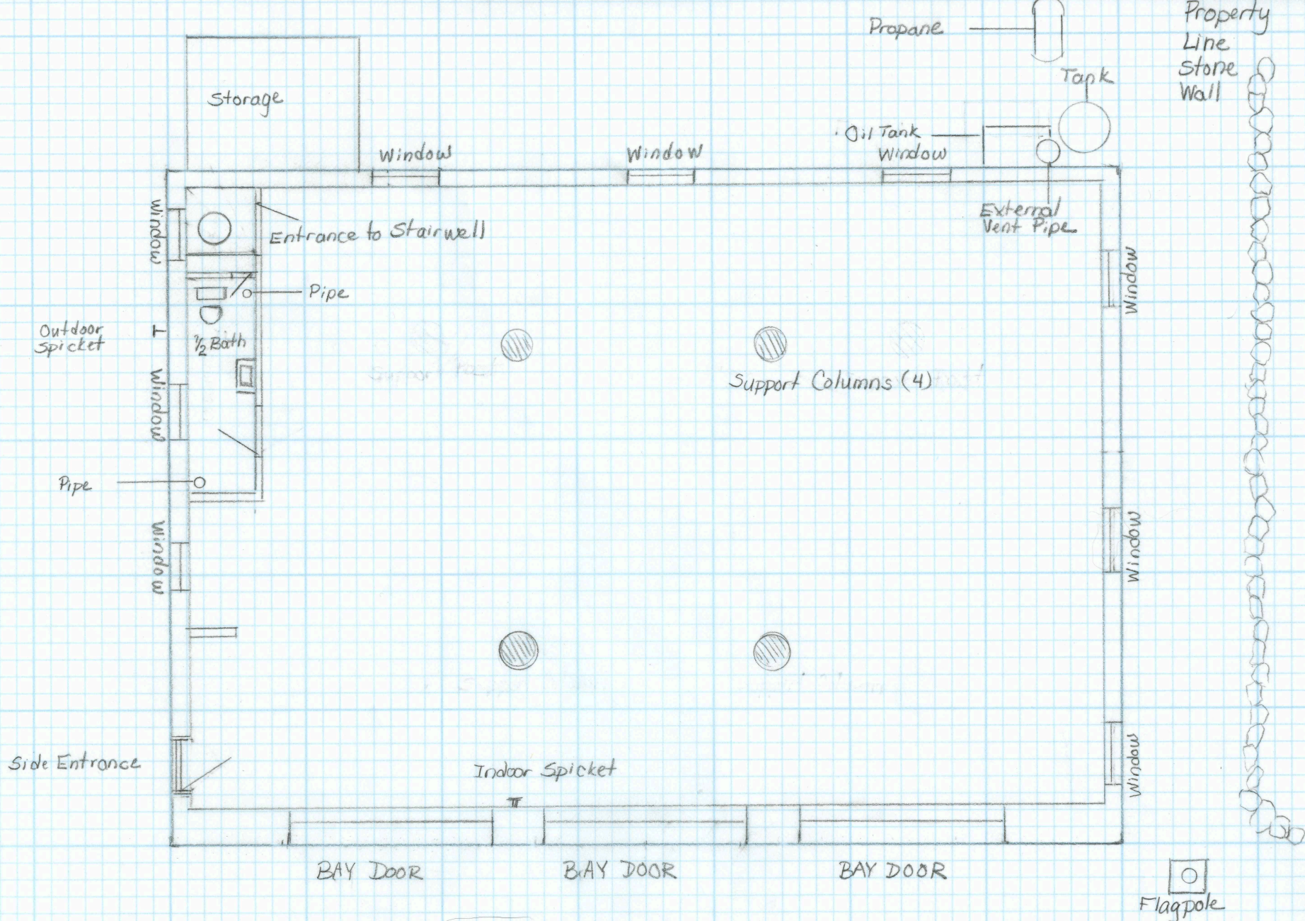
Old Mendon Fire Station Floor Plan First Floor Drive In Bays
